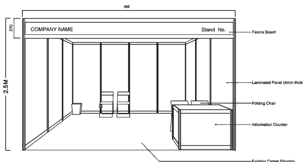
Perspective View (4.0mL x 3.0mW x 2.5mH)
