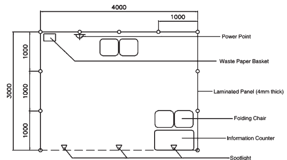
Vertical View (4.0mL x 3.0mW x 2.5mH)
